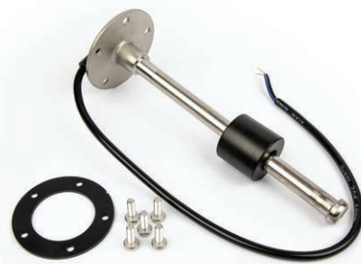
60L Flush Toilet Water Tank Sender (225mm)
