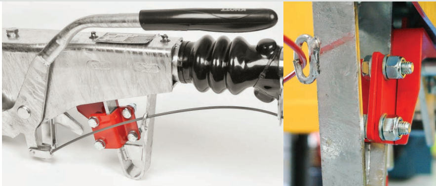
Bracket Kit Product Code: Type 1 = P260 | Type 2 = P264
