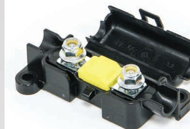
Midi Fused Holder for Sterling Charger
