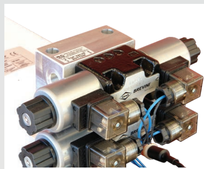
12 Volt Valve Block Solenoid (Top Mounted)
