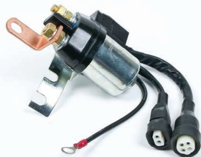
12 Volt Cylinder Start Solenoid (Side Mounted)
