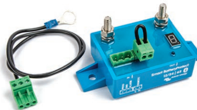
Victron Energy Smart BatteryProtect 12/24v-65A
